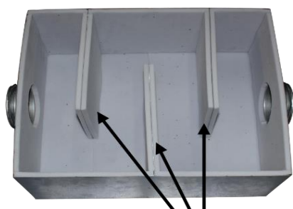
Chicane anti bruit Chicane Antilärm
